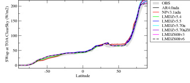
rsutcszone
