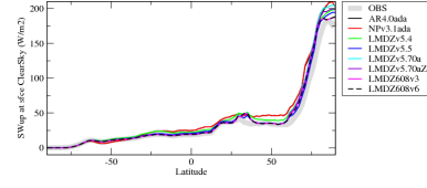
rsuscszone
