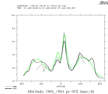
AR4.0ada_1982_1991_oce
