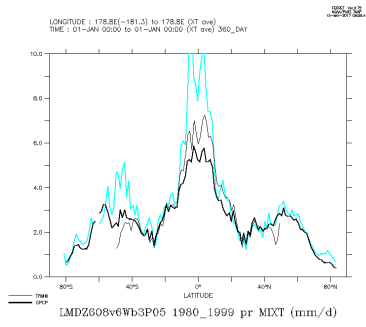
LMDZ608v6Wb3P05_1980_1999_mix
