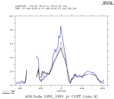
AR4.0ada_1982_1991_con
