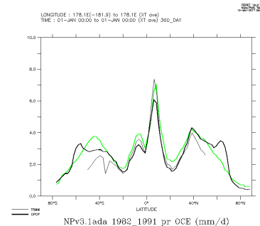
NPv3.1ada_1982_1991_oce
