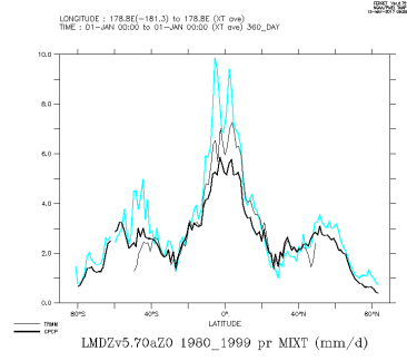
LMDZv5.70aZ0_1980_1999_mix
