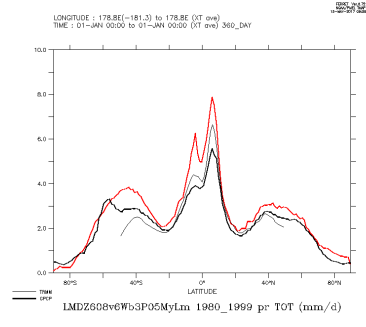
LMDZ608v6Wb3P05MyLm_1980_1999_tot
