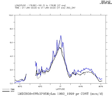
LMDZ608v6Wb3P05MyLm_1980_1999_con
