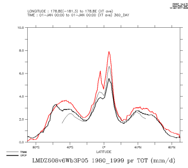
LMDZ608v6Wb3P05_1980_1999_tot
