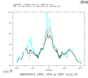
LMDZ608v3_1980_1999_mix
