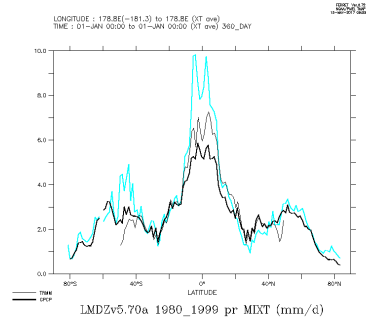
LMDZv5.70a_1980_1999_mix
