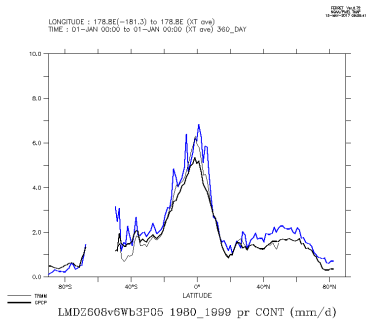
LMDZ608v6Wb3P05_1980_1999_con
