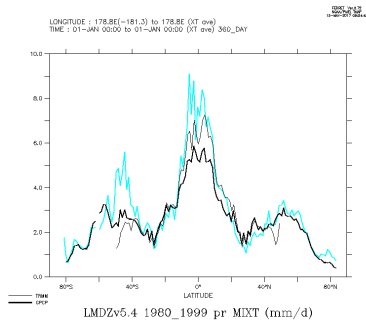
LMDZv5.4_1980_1999_mix
