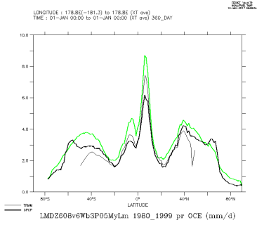
LMDZ608v6Wb3P05MyLm_1980_1999_oce
