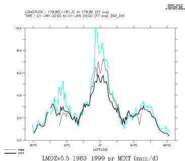
LMDZv5.5_1980_1999_mix
