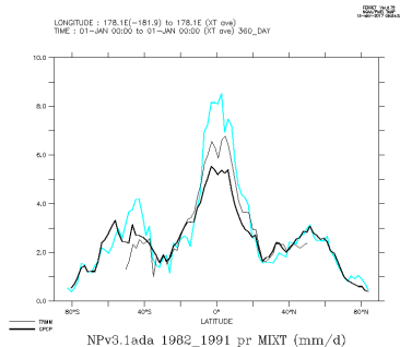
NPv3.1ada_1982_1991_mix
