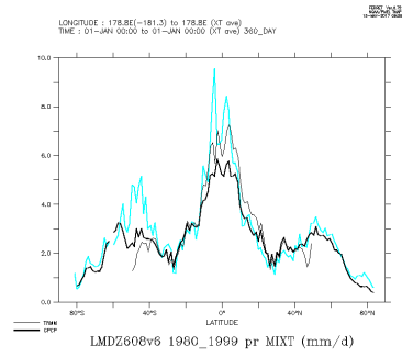
LMDZ608v6_1980_1999_mix
