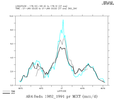
AR4.0ada_1982_1991_mix
