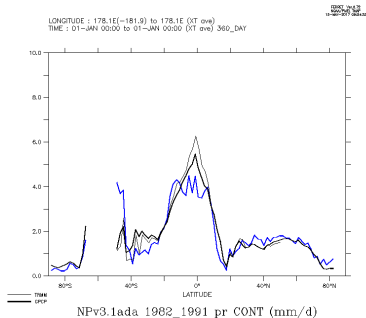
NPv3.1ada_1982_1991_con
