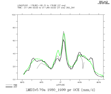
LMDZv5.70a_1980_1999_oce
