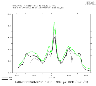
LMDZ608v6Wb3P05_1980_1999_oce
