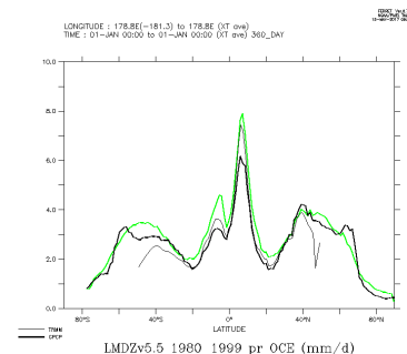
LMDZv5.5_1980_1999_oce
