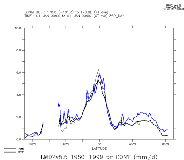
LMDZv5.5_1980_1999_con
