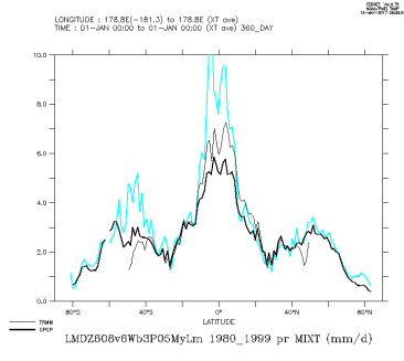
LMDZ608v6Wb3P05MyLm_1980_1999_mix
