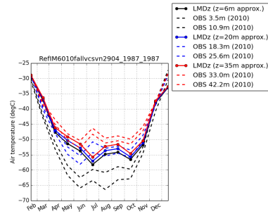
tempDC-RefIM6010fallvcsvn2904_1987_1987
