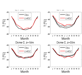
temp_DC_RefIM6010fallvcsvn2904_1987_1987
