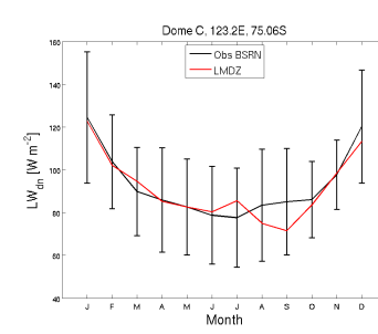
LWdnSFC_DC_RefIM607svn2904_1987_1987
