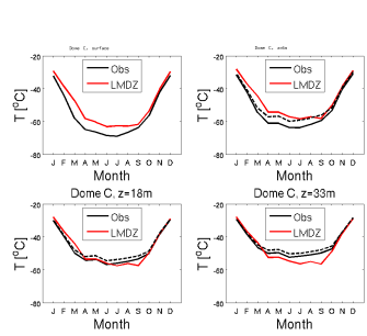
temp_DC_RefIM605svn2904_1987_1987
