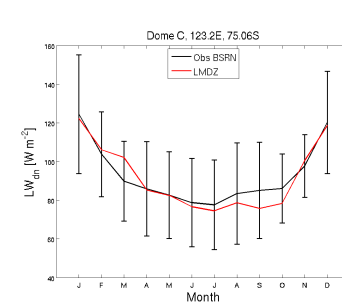
LWdnSFC_DC_RefIM605svn2904_1987_1987
