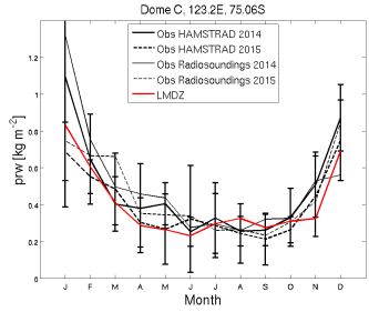
prw_DC-Wbm4.CLC20EPM95Epm2904_1987_1987
