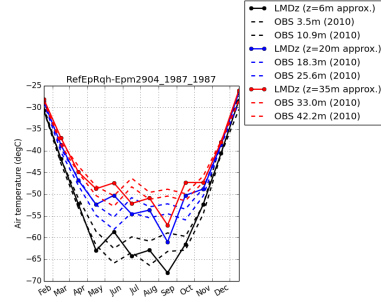
tempDC-RefEpRqh-Epm2904_1987_1987
