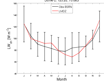
LWdnSFC_DC_RefIM609svn2904_1987_1987
