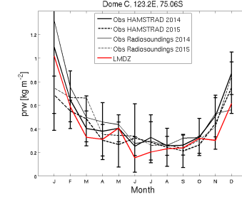
prw_DC_CLC09.EPM85blcv2904_1987_1987
