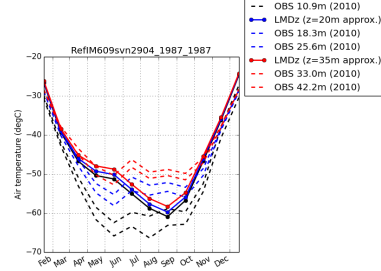
tempDC-RefIM609svn2904_1987_1987
