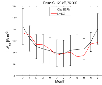
LWdnSFC_DC_RefIM6010fallvcsvn2904_1987_1987
