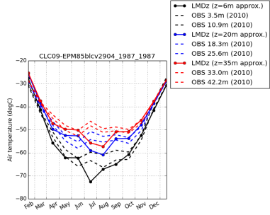
tempDC-CLC09-EPM85blcv2904_1987_1987
