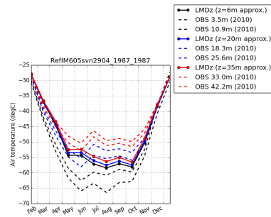
tempDC-RefIM605svn2904_1987_1987
