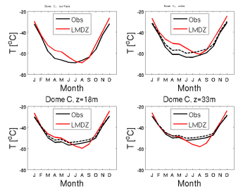
temp_DC_RefIM609svn2904_1987_1987
