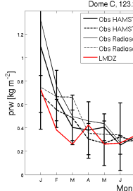
prw_DC_RefIM6010
