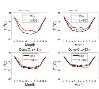
temp_DC_RefIM607svn2904_1987_1987
