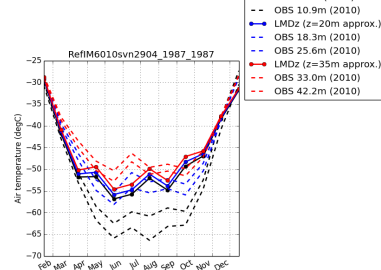
tempDC-RefIM6010svn2904_1987_1987
