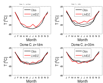
temp_DC_RefIM6010svn2904_1987_1987
