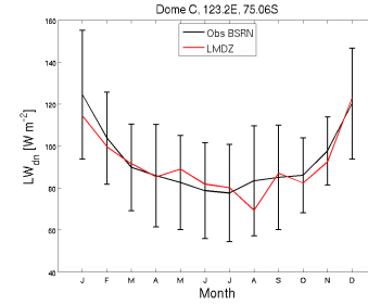
LWdnSFC_DC_RefEpRqh.Epm2904_1987_1987
