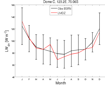
LWdnSFC_DC_CLC09.EPM85blcv2904_1987_1987
