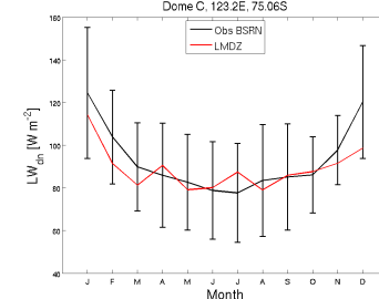
LWdnSFC_DC_RefIM6010svn2904_1987_1987
