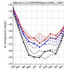
tempDC-Wbm4-CLC20EPM95Epm2904_1987_1987
