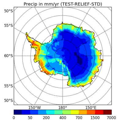
precipSH-TEST-RELIEF-STD
