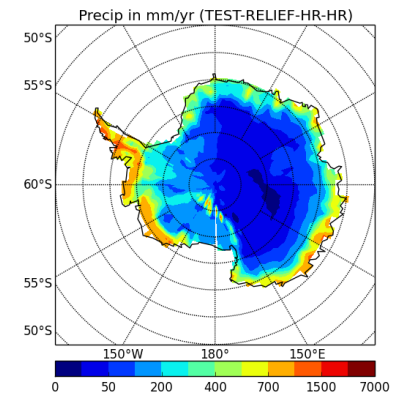
precipSH-TEST-RELIEF-HR-HR
