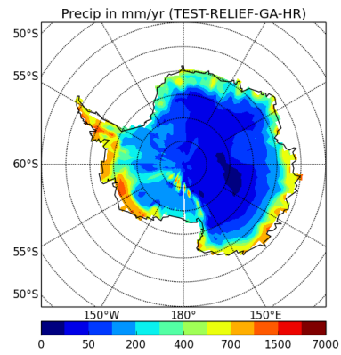
precipSH-TEST-RELIEF-GA-HR
