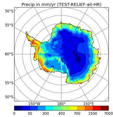
precipSH-TEST-RELIEF-all-HR
