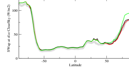
rsuscson
