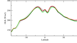
rlutzon
