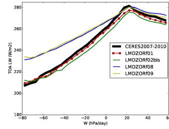
rlut_NuagesHauts
