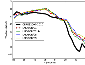
rtt_NuagesHauts
