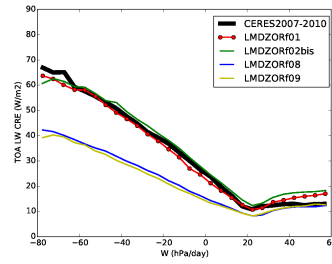
cretl_NuagesHauts
