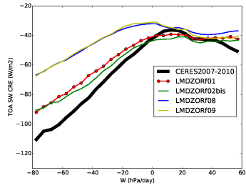
crest_NuagesHauts
