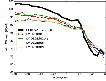
rsah_NuagesHauts
