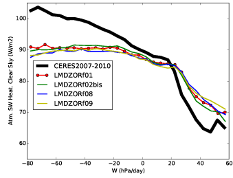
rsahcs_NuagesHauts
