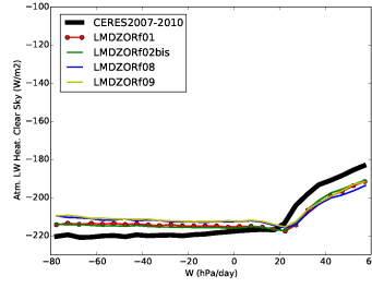
rlahcs_NuagesHauts
