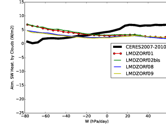
rsahcre_NuagesHauts
