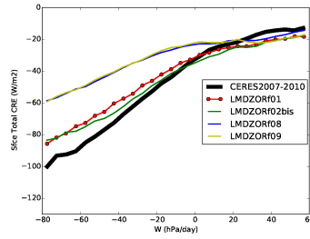
cretts_NuagesHauts
