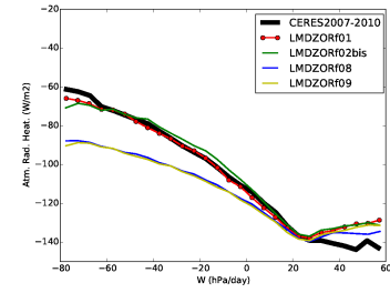
rah_NuagesHauts
