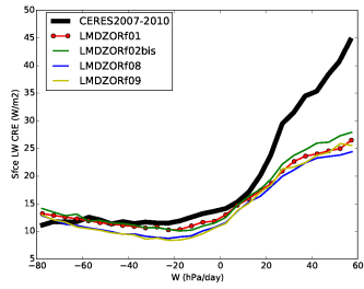
crels_NuagesHauts
