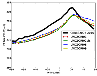
rlutcs_NuagesHauts
