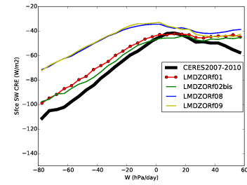
cress_NuagesHauts
