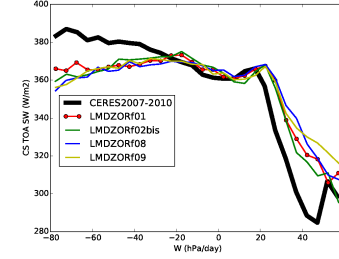
rsttcs_NuagesHauts
