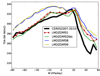
rstt_NuagesHauts
