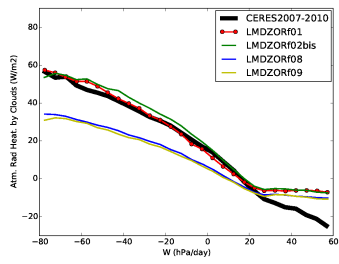
rahcre_NuagesHauts
