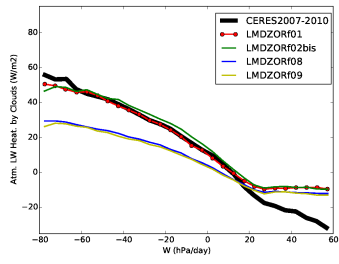
rlahcre_NuagesHauts
