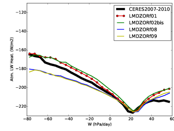
rlah_NuagesHauts
