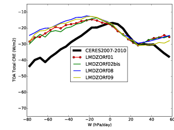
crettt_NuagesHauts
