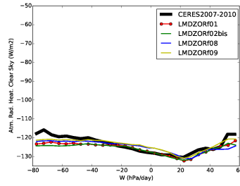
rahcs_NuagesHauts
