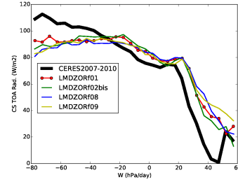
rttcs_NuagesHauts
