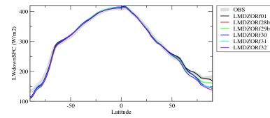
rldsazon
