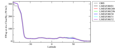
rsuscson
