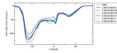
crestzon
