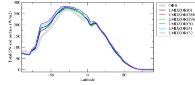
rsdsazon
