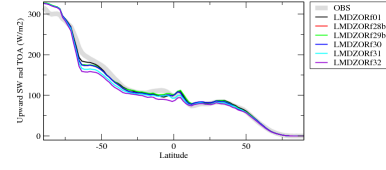
rsutazon
