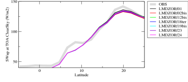
rsuscscszon
