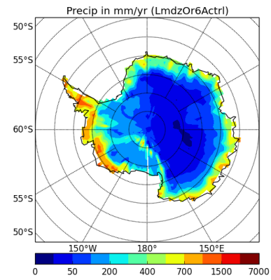
precipSH-LmdzOr6Actrl
