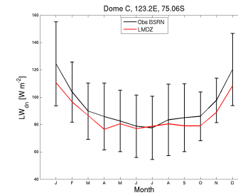
Missing tsol_DC_LmdzOrAPctrl.1990_1999
