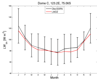
Missing tsol_DC_LmdzOrChoi6A_1990_1999
