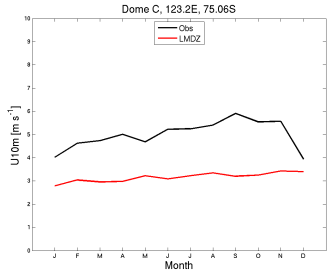
wind10m_DC_LmdzOrRsoil6A_1990_1999
