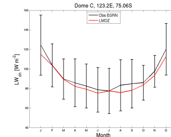
Missing tsol_DC_LmdzOrRsoil6A_1990_1999
