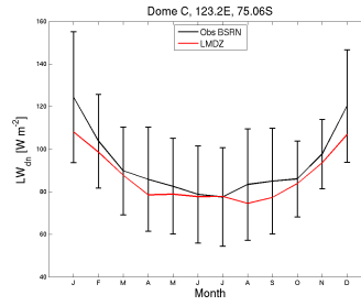
Missing tsol_DC_LmdzOr6AnoFreeznoExplsnow_1990_1999
