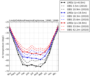
tempDC-LmdzOr6AnoFreeznoExplsnow_1990_1999
