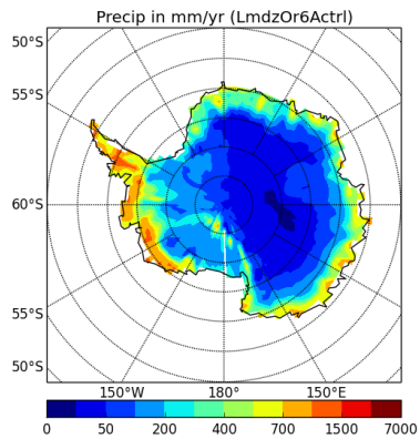
precipSH-LmdzOr6Actrl
