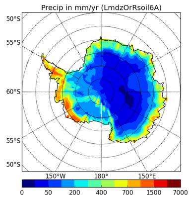
precipSH-LmdzOrRsoil6A
