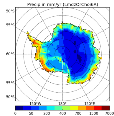
precipSH-LmdzOrChoi6A
