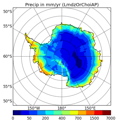
precipSH-LmdzOrChoiAP
