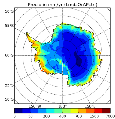
precipSH-LmdzOrAPctrl
