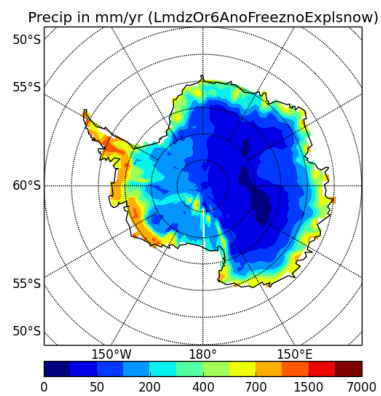
precipSH-LmdzOr6AnoFreeznoExplsnow
