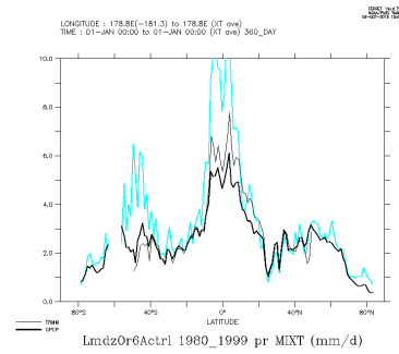
LmdzOr6Actrl_1980_1999_mix
