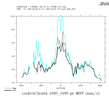
LmdzOrChoi6A_1980_1999_mix
