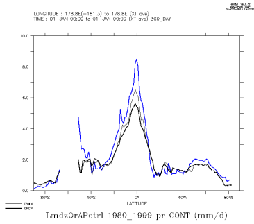
LmdzOrAPctrl_1980_1999_con
