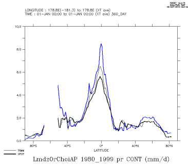
LmdzOrChoiAP_1980_1999_con
