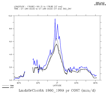
LmdzOrChoi6A_1980_1999_con
