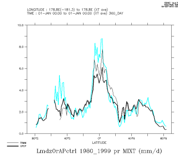
LmdzOrAPctrl_1980_1999_mix
