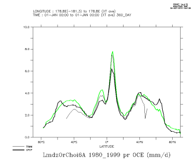
LmdzOrChoi6A_1980_1999_oce
