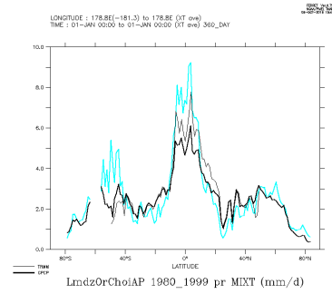
LmdzOrChoiAP_1980_1999_mix
