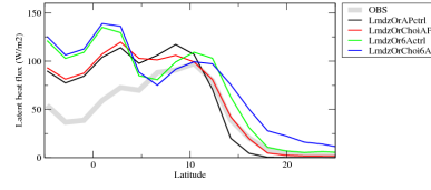
hfsfzon
