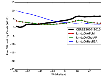
rsahcre_LmdzOr11et2cAP
