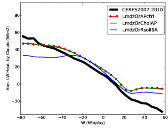
rlahcre_LmdzOr11et2cAP
