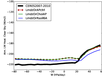
rlahcs_LmdzOr11et2cAP
