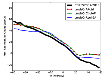
rahcre_LmdzOr11et2cAP
