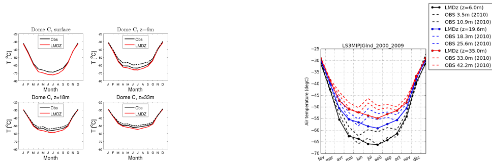
temp_DC_LS3MIPJGlnl_2000_2009
