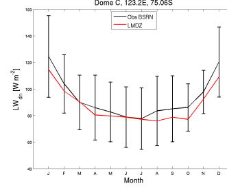
LWdnSFC_DC_LS3MIPJGlnDg_2000_2009
