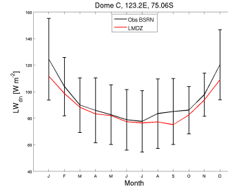
LWdnSFC_DC_LS3MIPJGlnD_2000_2009
