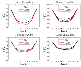
temp_DC_LS3MIPJGlnDg_2000_2009
