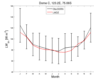
LWdnSFC_DC_LS3MIPJG_1999_2008
