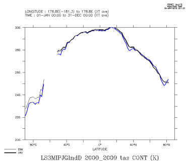
LS3MIPJGlnD_2000_2009_con
