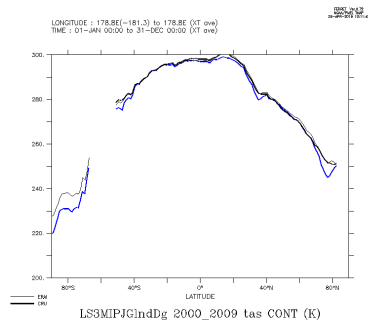
LS3MIPJGlnDg_2000_2009_con
