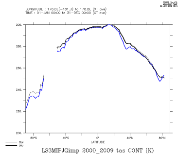
LS3MIPJGimp_2000_2009_con
