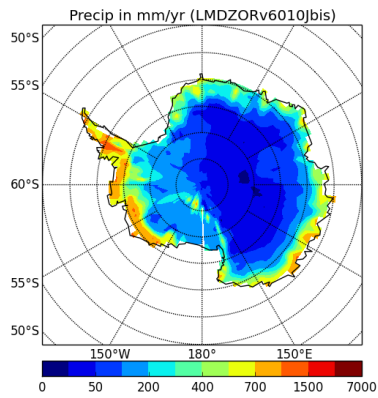
precipSH-LMDZORv6010Jbis
