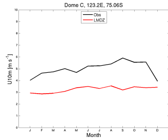
wind10m_DC_CM6.0.14splith_1980_1989
