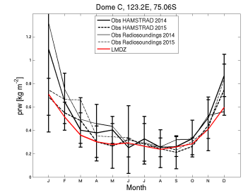
LWdnSFC_DC_CM6.0.14splith_1980_1989
