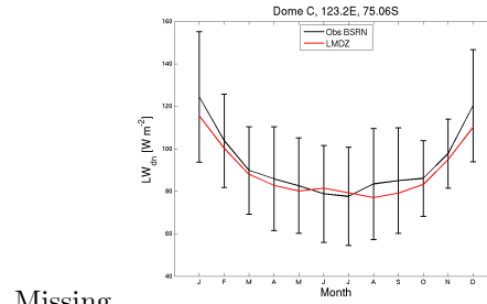
Missing tsol_DC_CM6.0.14splith_1980_1989
