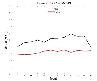
wind10m_DC_CM6.0.14splithBug_1980_1989
