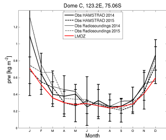
prw_DC_CM6.0.14splithBug_1980_1989
