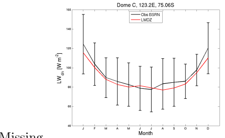
Missing tsol_DC_CM6.0.14splithBug_1980_1989
