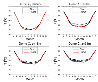
temp_DC_CM6.0.14splithBug_1980_1989
