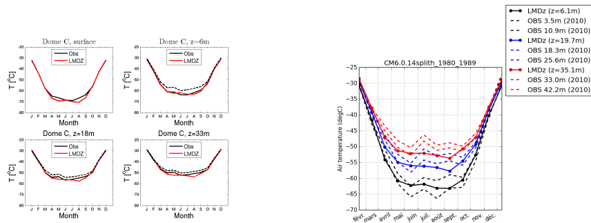
temp_DC_CM6.0.14splith_1980_1989
