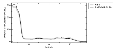
rsuscszon
