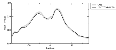
rlutzon
