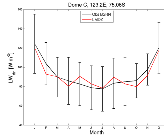
tsol_DC_LMDZOR6AT01_1980_1980
