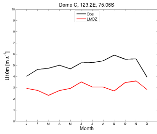
wind10m_DC_LMDZOR6AT01_1980_1980
