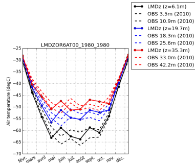
tempDC-LMDZOR6AT00_1980_1980
