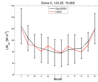
tsol_DC_LMDZOR6AT00_1980_1980
