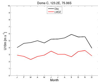
wind10m_DC_LMDZOR6AT00_1980_1980
