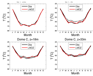
temp_DC_LMDZOR6AT00_1980_1980
