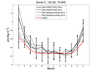
prw_DC_LMDZOR14httop_1980.1989
