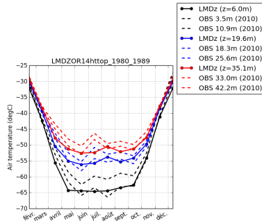
tempDC-LMDZOR14httop_1980.1989
