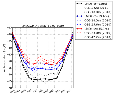
tempDC-LMDZOR14splitD_1980-1989
