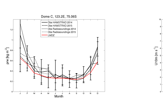
prw_DC_LMDZOR14splitD_1980-1989
