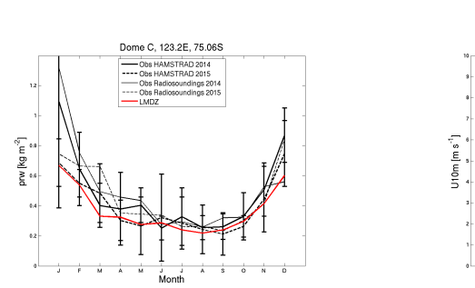
prw_DC_LMDZOR14splith_1980-1989
