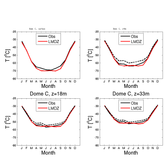
temp_DC_LMDZOR14splitD_1980-1989
