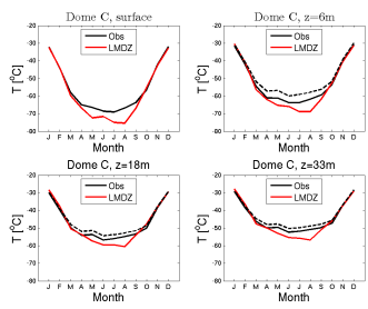
temp_DC_LMDZORv6011ttop_1980_1984
