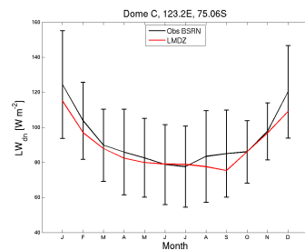
LWdnSFC_DC_LMDZORv6011pmagicH_1980_1984
