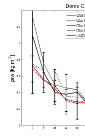
prw_DC_LMDZORv6011split_1980_1984
