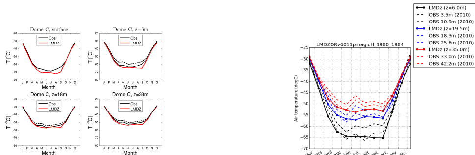
temp_DC_LMDZORv6011pmagicH_1980_1984
