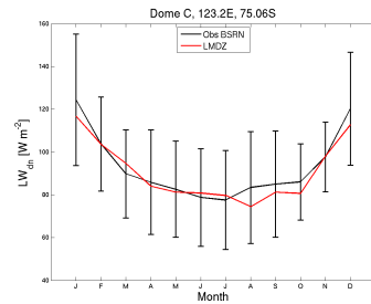
LWdnSFC_DC_LMDZORv6011split_1980_1984
