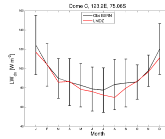
LWdnSFC_DC_LMDZORv6011ttop_1980_1984
