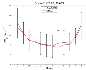
LWdnSFC_DC_LMDZORv6011cvoroF_1980_1984
