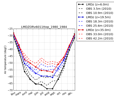
tempDC-LMDZORv6011ttop_1980_1984
