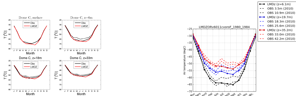
temp_DC_LMDZORv6011cvoroF_1980_1984
