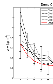
prw_DC_LMDZORv6011pmagicH_1980_1984
