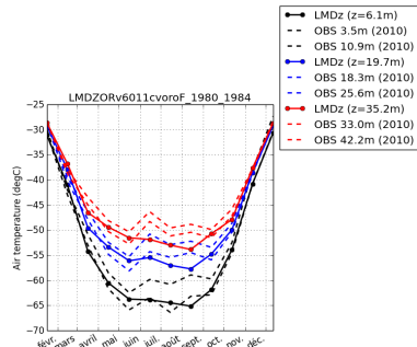
tempDC-LMDZORv6011cvoroF_1980_1984
