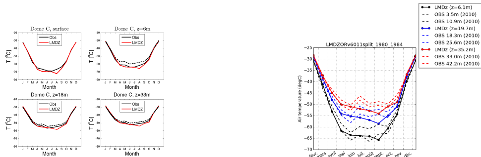
temp_DC_LMDZORv6011split_1980_1984
