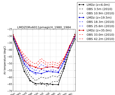
tempDC-LMDZORv6011pmagicH_1980_1984
