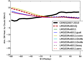
rsahcre_LMDZOR6011
