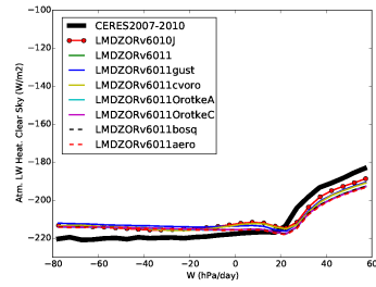
rlahcs_LMDZOR6011
