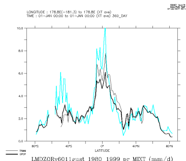
LMDZORv6011gust_1980_1999_mix
