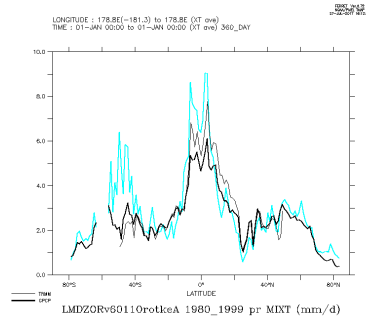
LMDZORv6011OrotkeA.1980_1999_mix
