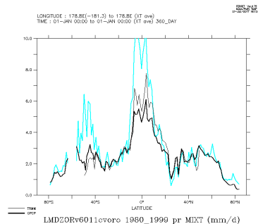
LMDZORv6011cvoro_1980_1999_mix
