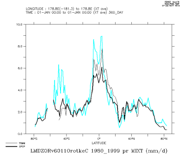
LMDZORv6011OrotkeC.1980_1999_mix
