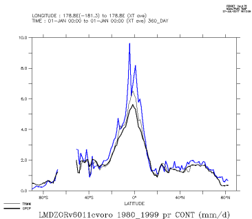
LMDZORv6011cvoro_1980_1999_con
