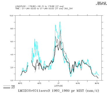
LMDZORv6011aeroB.1980_1989_mix
