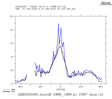
LMDZORv6011aeroB.1980_1989_con
