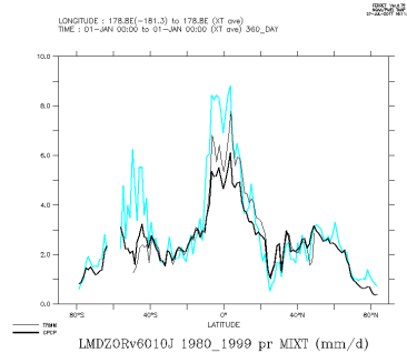
LMDZORv6010J_1980_1999_mix
