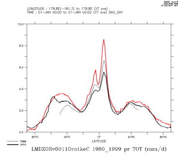
LMDZORv6011OrotkeC.1980_1999_tot
