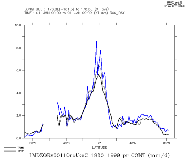
LMDZORv6011OrotkeC.1980_1999_con
