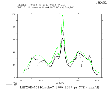
LMDZORv6011OrotkeC.1980_1999_oce
