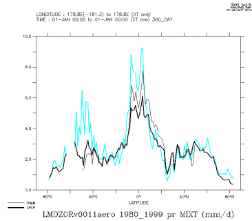
LMDZORv6011aero.1980_1999_mix
