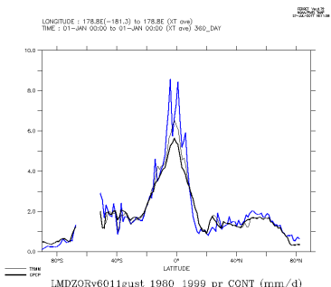
LMDZORv6011gust_1980_1999_con
