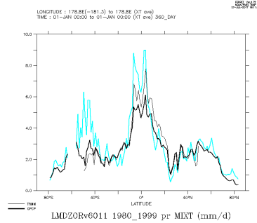
LMDZORv6011_1980_1999_mix
