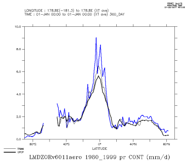
LMDZORv6011aero.1980_1999_con
