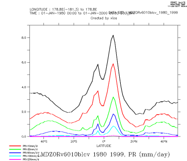
LMDZORv6010blcv_1980_1999_zon
