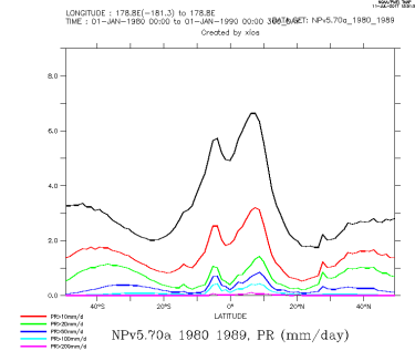
NPv5.70a_1980_1989_zon
