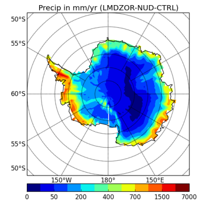
precipSH-LMDZOR-NUD-CTRL
