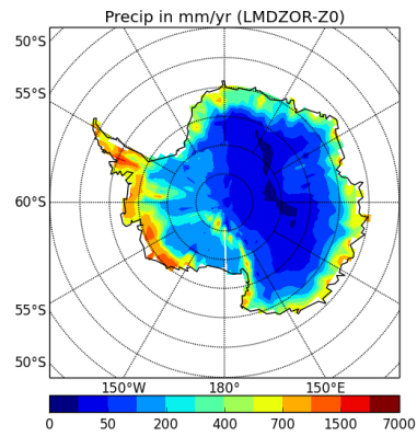
precipSH-LMDZOR-Z0
