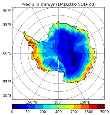
precipSH-LMDZOR-NUD-Z0
