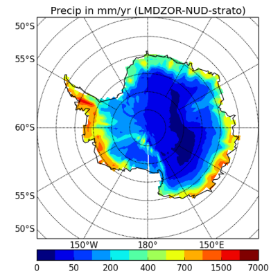
precipSH-LMDZOR-NUD-strato
