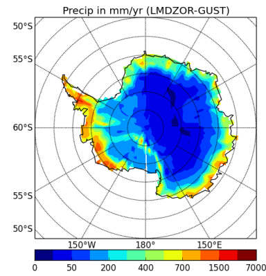
precipSH-LMDZOR-GUST
