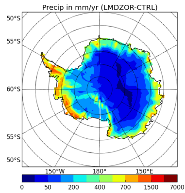
precipSH-LMDZOR-CTRL
