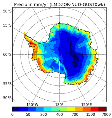
precipSH-LMDZOR-NUD-GUST0wk
