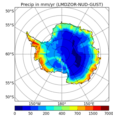
precipSH-LMDZOR-NUD-GUST
