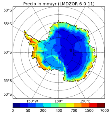
precipSH-LMDZOR-6-0-11
