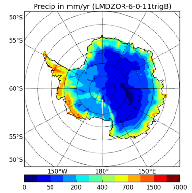
precipSH-LMDZOR-6-0-11trigB
