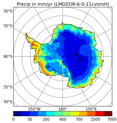
precipSH-LMDZOR-6-0-11cvoroH
