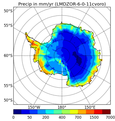
precipSH-LMDZOR-6-0-11cvoro
