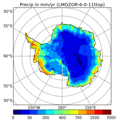
precipSH-LMDZOR-6-0-11ttop
