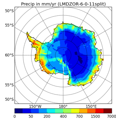
precipSH-LMDZOR-6-0-11split
