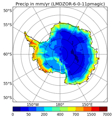
precipSH-LMDZOR-6-0-11pmagic
