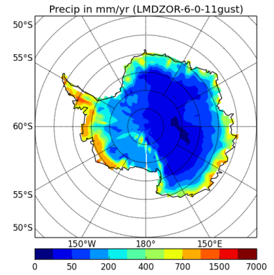
precipSH-LMDZOR-6-0-11gust
