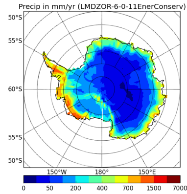
precipSH-LMDZOR-6-0-11EnerConserv
