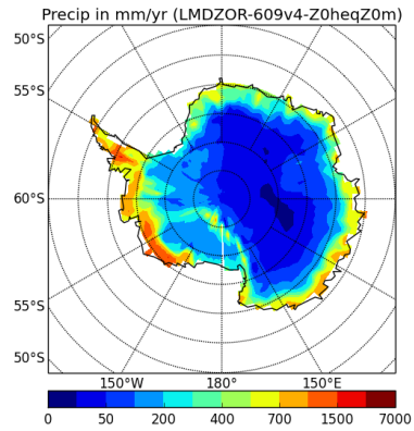
precipSH-LMDZOR-609v4-Z0heqZ0m
