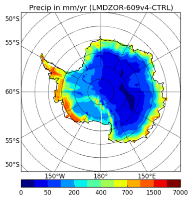
precipSH-LMDZOR-609v4-CTRL
