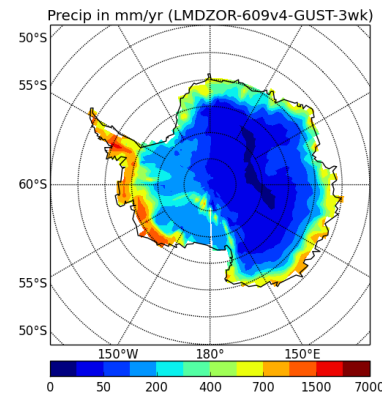
precipSH-LMDZOR-609v4-GUST-3wk
