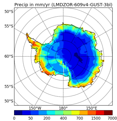
precipSH-LMDZOR-609v4-GUST-3bl
