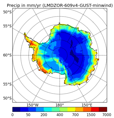
precipSH-LMDZOR-609v4-GUST-minwind
