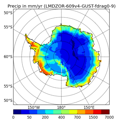
precipSH-LMDZOR-609v4-GUST-fdrag0-9
