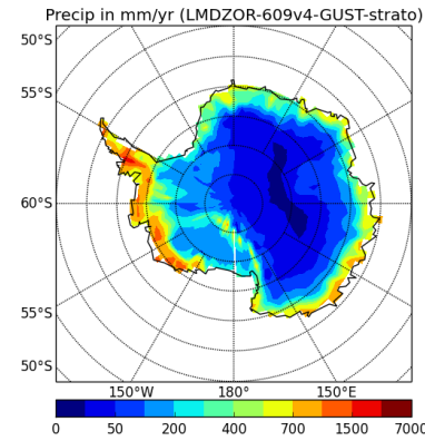
precipSH-LMDZOR-609v4-GUST-strato
