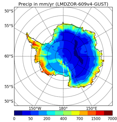
precipSH-LMDZOR-609v4-GUST
