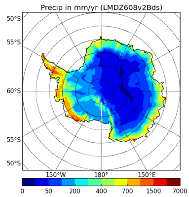
precipSH-LMDZ608v2Bds
