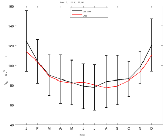
LWdn_DC_LMDZ608v6Wb3P05MyLmGust_1980_1999
