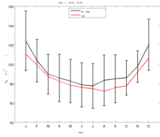
LWdn_DC_LMDZ608v6oro_1980_1999
