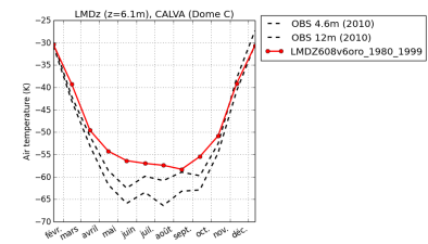
tempDC-LMDZ608v6oro_1980_1999
