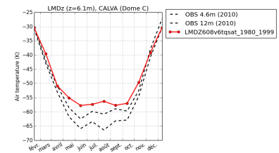
tempDC-LMDZ608v6tqsat_1980_1999
