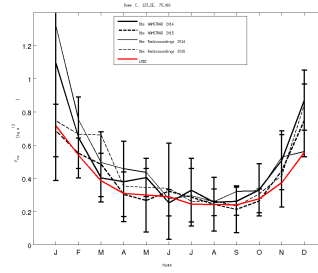
prw_DC_LMDZ608v6Wb3P05MyLm_1980_1999
