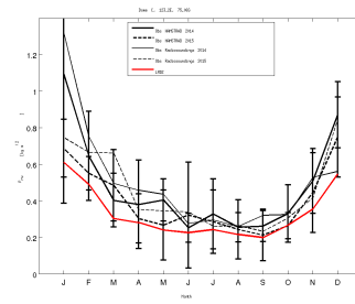
prw_DC_LMDZ608v6tqsat_1980_1999
