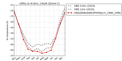
tempDC-LMDZ608v6Wb3P05MyLm_1980_1999
