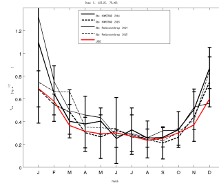
prw_DC_LMDZ608v6Wb3P05MyLmGust_1980_1999
