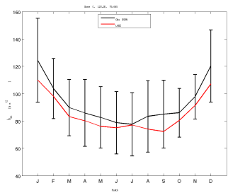
LWdn_DC_LMDZ608v6tqsat_1980_1999
