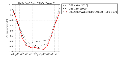
tempDC-LMDZ608v6Wb3P05MyLmGust_1980_1999
