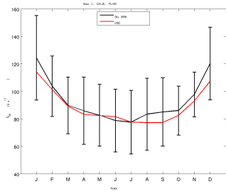
LWdn_DC_LMDZ608v6Wb3P05MyLm_1980_1999
