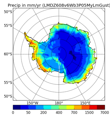
precipSH-LMDZ608v6Wb3P05MyLmGust
