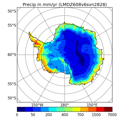
precipSH-LMDZ608v6svn2828
