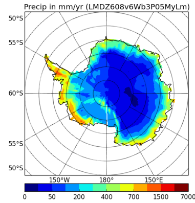
precipSH-LMDZ608v6Wb3P05MyLm
