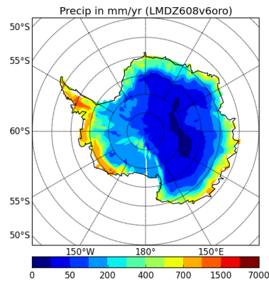
precipSH-LMDZ608v6oro
