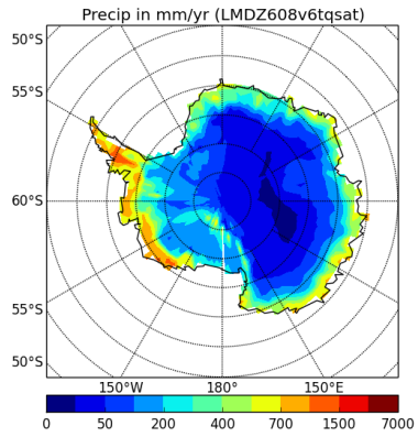
precipSH-LMDZ608v6tqsat
