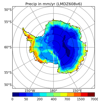
precipSH-LMDZ608v6
