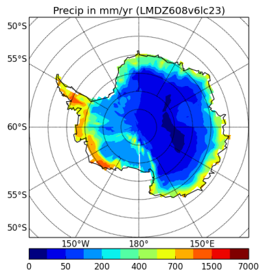
precipSH-LMDZ608v6lc23
