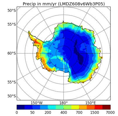
precipSH-LMDZ608v6Wb3P05
