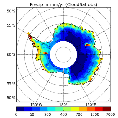
precipSH-OBS
