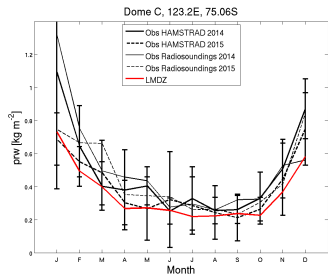
prw_DC_CM6011.3-LR-amip-ttop-G-02_1999_2008
