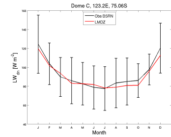
tsoL_DC_CM6011.3-LR-amip-G-02_1999_2008
