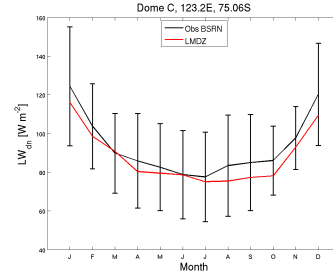
Missing tsol_DC_CM6011.3-LR-amip-trigB-G-02_1999_2008
