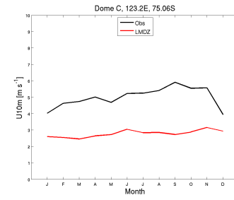
prw_DC_CM6011.3-LR-amip-split-G-02_1999_2008
