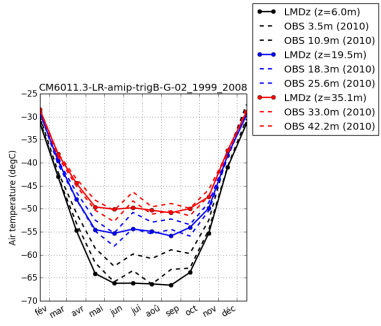
tempDC_CM6011.3-LR-amip-trigB-G-02_1999_2008
