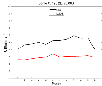
wind10m_DC_CM6011.3-LR-amip-G-02_1999_2008
