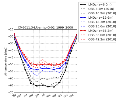
tempDC_CM6011.3-LR-amip-G-02_1999_2008
