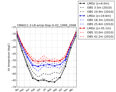
tempDC_CM6011.3-LR-amip-ttop-G-02_1999_2008
