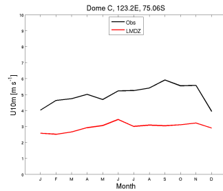
wind10m_DC_CM6011.3-LR-amip-ttop-G-02_1999_2008
