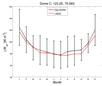
Missing tsol_DC_CM6011.3-LR-amip-split-G-02_1999_2008
