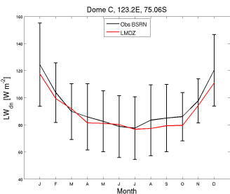
LWdnSFC_DC_CM6011.3-LR-amip-cvoroH-G-02_1999_2008
