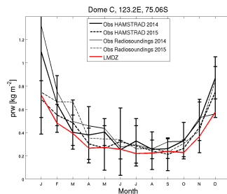
prw_DC_CM6011.3-LR-amip-cvoroH-G-02_1999_2008
