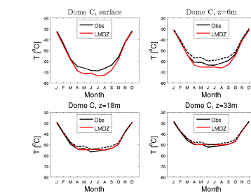
temp_DC_CM6011.3-LR-amip-cvoroH-G-02_1999_2008
