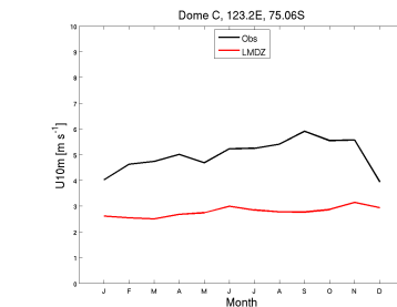
wind10m_DC_CM6011.3-LR-amip-cvoroH-G-02_1999_2008
