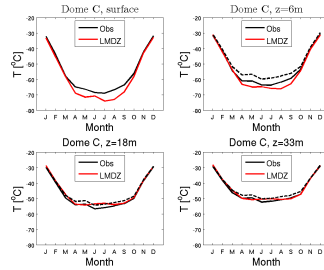
temp_DC_CM6011.3-LR-amip-ttop-G-02_1999_2008
