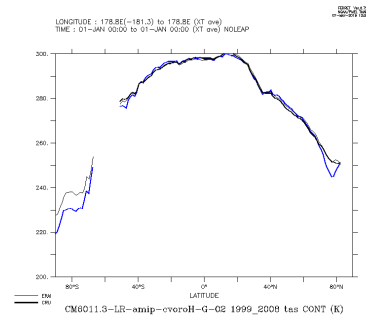
CM6011.3-LR-amip-cvoroH-G-02_1999_2008.con
