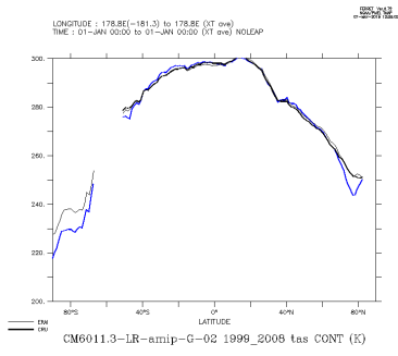
CM6011.3-LR-amip-G-02_1999_2008.con
