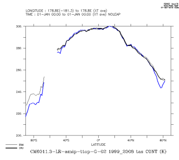
CM6011.3-LR-amip-ttop-G-02_1999_2008.con
