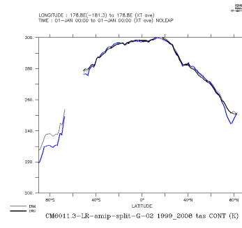
CM6011.3-LR-amip-split-G-02_1999_2008.con
