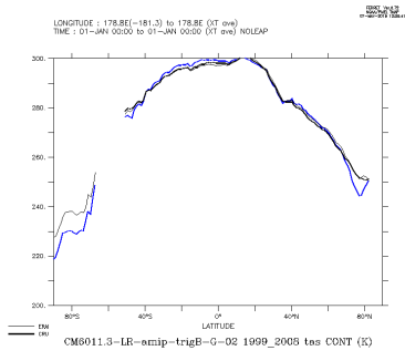
CM6011.3-LR-amip-trigB-G-02_1999_2008.con
