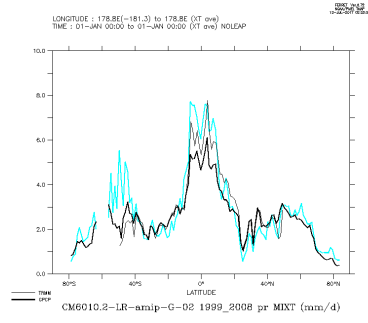
CM6010.2-LR-amp-G-02_1999_2008.mix
