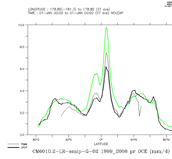
CM6010.2-LR-amp-G-02_1999_2008.oce
