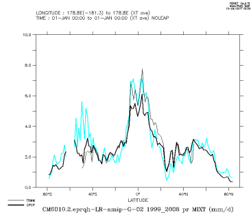
CM6010.2.eprqh-LR-amip-G-02_1999_2008_mix
