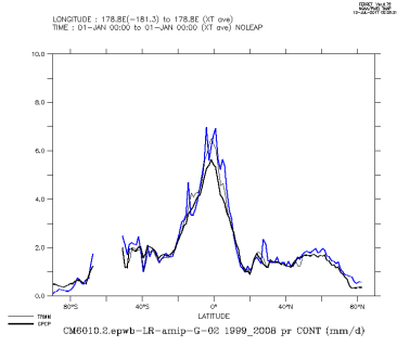
CM6010.2.epwb-LR-amip-G-02_1999_2008_con
