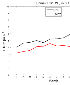
wind10m_DC_CM609-LR-amip-G-01_1999_2008
