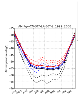
tempDC-AMIPgv-CM607-LR-30Y-2_1999_2008
