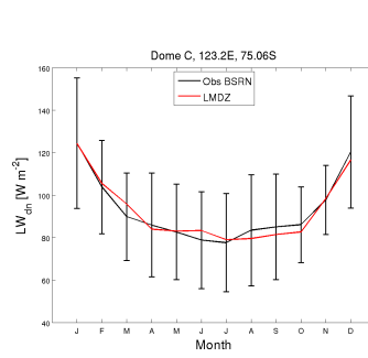
LWdnSFC_DC_AMIPg.vt-CM607-LR.2_1999_2008
