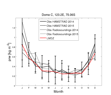
prw_DC_AMIPgv-CM607-LR.30Y.2_1999_2008
