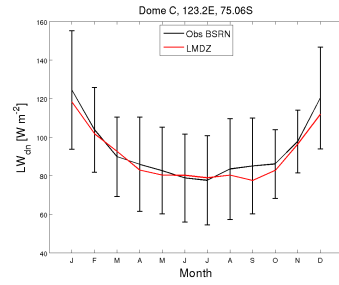
LWdnSFC_DC_AMIP-CM607-LR.30Y.2_1999_2008
