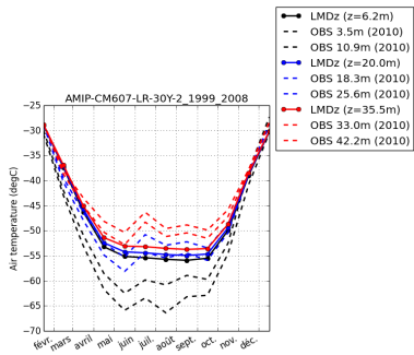
tempDC-AMIP-CM607-LR-30Y-2_1999_2008
