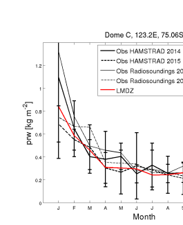
prw_DC_AMIPg.vt-CM607-LR.2_1999_2008
