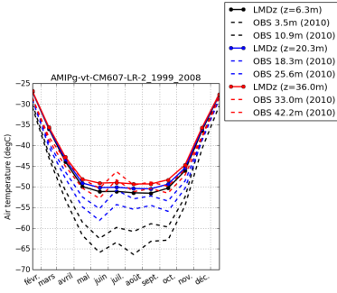
tempDC-AMIPg-vt-CM607-LR-2_1999_2008
