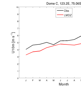
wind10m_DC_CM608-LR-amip-01_1999_2008
