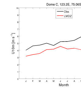
wind10m_DC_CM608-LR-amip-G-01_1999_2008
