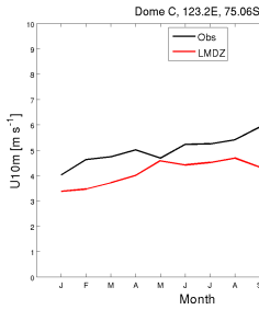
wind10m_DC_CM609-LR-amip-01_1999_2008
