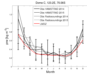
prw_DC_AMIP-CM607-LR.30Y.2_1999_2008
