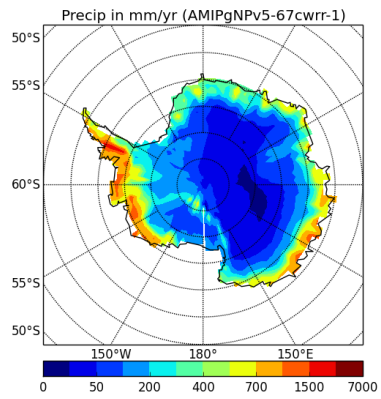
precipSH-AMIPgNPv5-67cwrr-1
