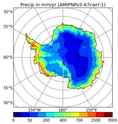
precipSH-AMIPNPv5-67cwrr-1
