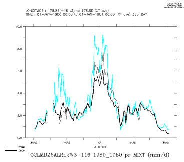
Q2LMDZ6ALRE2W3-116.1980_1980_mix
