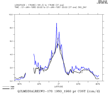
Q2LMDZ6ALRE2W3-170_1980_1980_con
