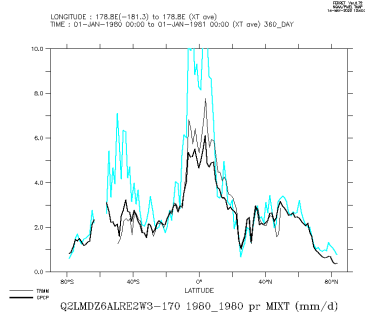
Q2LMDZ6ALRE2W3-170_1980_1980_mix
