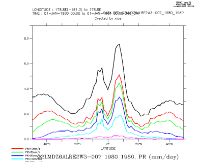
Q2LMDZ6ALRE2W3-007_1980_1980_zon
