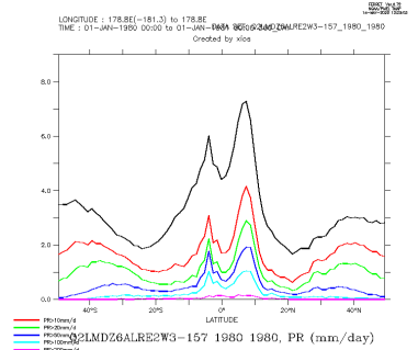
Q2LMDZ6ALRE2W3-157_1980_1980_zon
