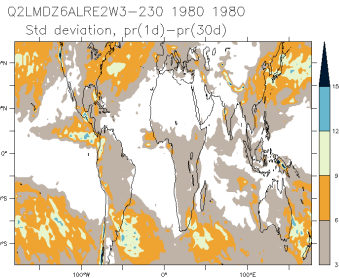
Q2LMDZ6ALRE2W3-230_1980_1980_hf
