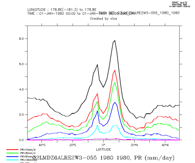
Q2LMDZ6ALRE2W3-055_1980_1980_zon
