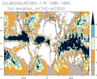
Q2LMDZ6ALRE2W3-176_1980_1980_hf
