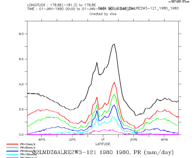
Q2LMDZ6ALRE2W3-121_1980_1980_zon
