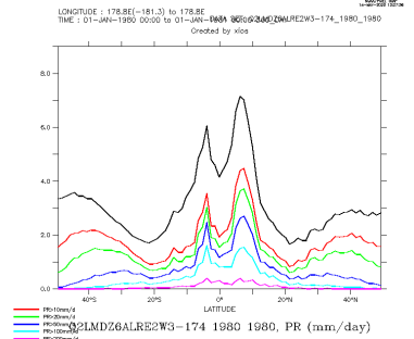
Q2LMDZ6ALRE2W3-174_1980_1980_zon
