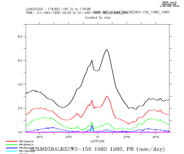
Q2LMDZ6ALRE2W3-156_1980_1980_zon
