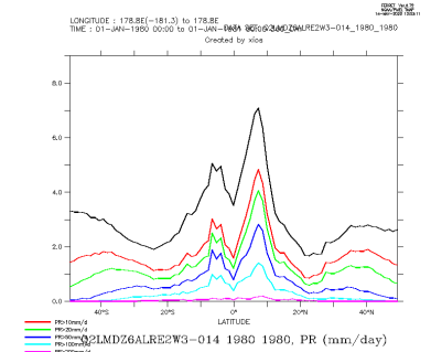
Q2LMDZ6ALRE2W3-014_1980_1980_zon
