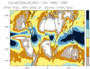
Q2LMDZ6ALRE2W3-104_1980_1980_nd
