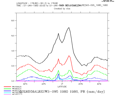
Q2LMDZ6ALRE2W3-095_1980_1980_zon
