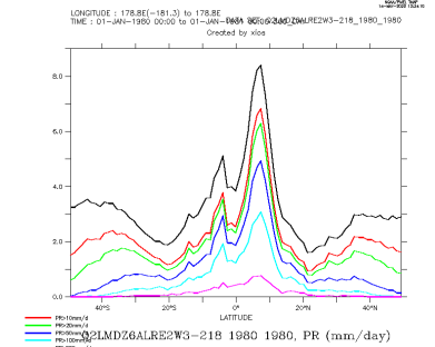
Q2LMDZ6ALRE2W3-218_1980_1980_zon
