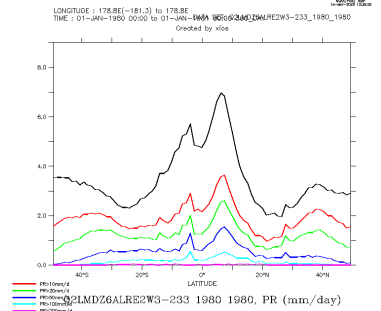
Q2LMDZ6ALRE2W3-233_1980_1980_zon
