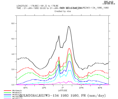
Q2LMDZ6ALRE2W3-134_1980_1980_zon
