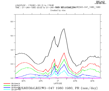
Q2LMDZ6ALRE2W3-047_1980_1980_zon
