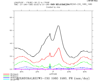
Q2LMDZ6ALRE2W3-230_1980_1980_zon
