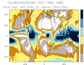
Q2LMDZ6ALRE2W3-007_1980_1980_nd
