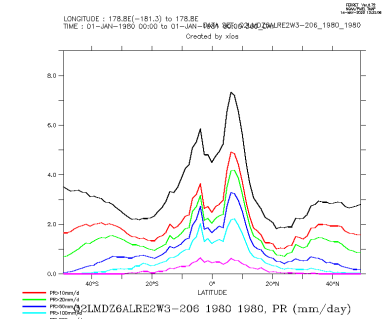
Q2LMDZ6ALRE2W3-206_1980_1980_zon
