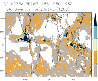
Q2LMDZ6ALRE2W3-185_1980_1980_is
