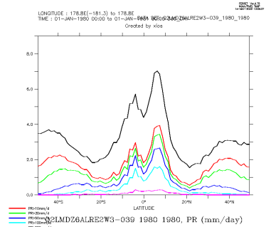
Q2LMDZ6ALRE2W3-039_1980_1980_zon
