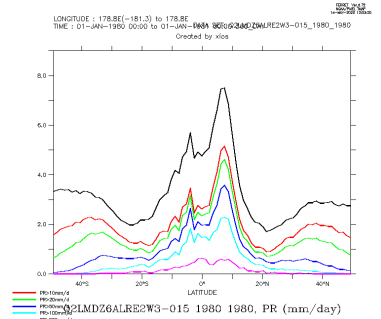
Q2LMDZ6ALRE2W3-015_1980_1980_zon
