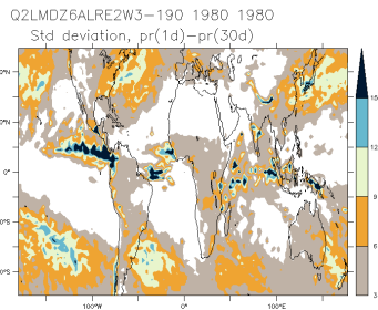
Q2LMDZ6ALRE2W3-190_1980_1980_hf
