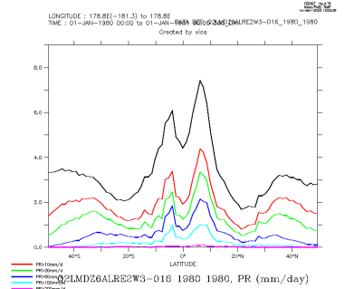
Q2LMDZ6ALRE2W3-016_1980_1980_zon
