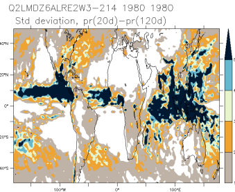
Q2LMDZ6ALRE2W3-214_1980_1980_is
