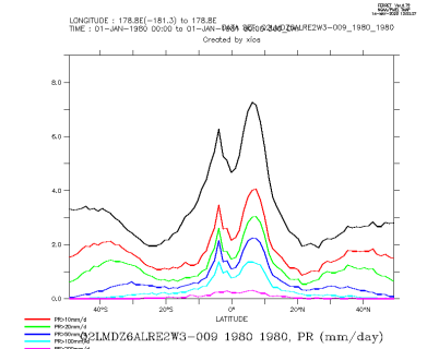
Q2LMDZ6ALRE2W3-009_1980_1980_zon
