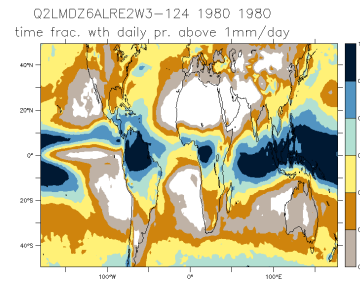
Q2LMDZ6ALRE2W3-124_1980_1980_nd
