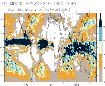
Q2LMDZ6ALRE2W3-210_1980_1980_hf
