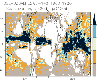
Q2LMDZ6ALRE2W3-140_1980_1980_is
