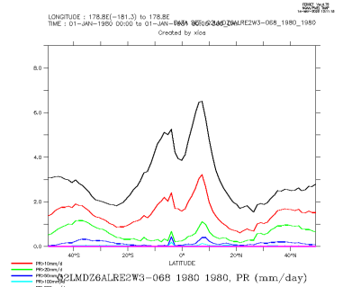
Q2LMDZ6ALRE2W3-068_1980_1980_zon
