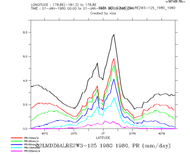
Q2LMDZ6ALRE2W3-125_1980_1980_zon
