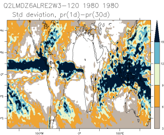
Q2LMDZ6ALRE2W3-120_1980_1980_hf
