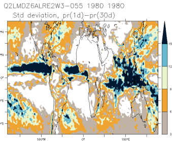
Q2LMDZ6ALRE2W3-055_1980_1980_hf
