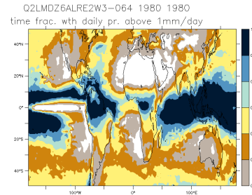
Q2LMDZ6ALRE2W3-064_1980_1980_nd
