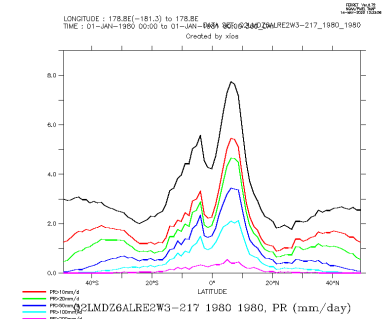
Q2LMDZ6ALRE2W3-217_1980_1980_zon
