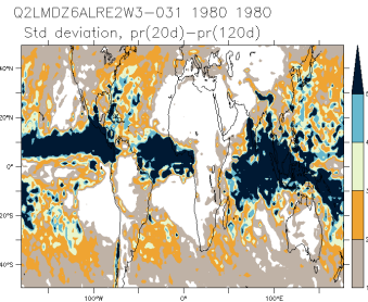
Q2LMDZ6ALRE2W3-031_1980_1980_is
