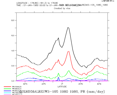
Q2LMDZ6ALRE2W3-105_1980_1980_zon
