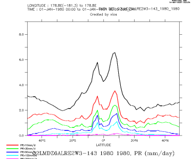
Q2LMDZ6ALRE2W3-143_1980_1980_zon
