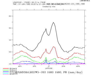
Q2LMDZ6ALRE2W3-203_1980_1980_zon
