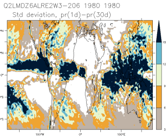
Q2LMDZ6ALRE2W3-206_1980_1980_hf
