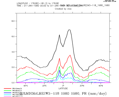
Q2LMDZ6ALRE2W3-118_1980_1980_zon
