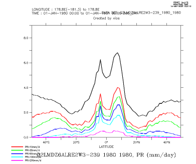
Q2LMDZ6ALRE2W3-239_1980_1980_zon
