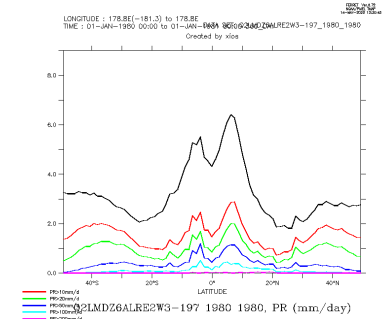
Q2LMDZ6ALRE2W3-197_1980_1980_zon
