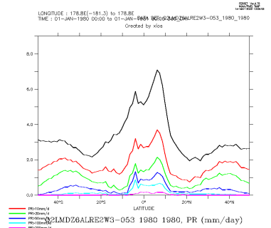
Q2LMDZ6ALRE2W3-053_1980_1980_zon
