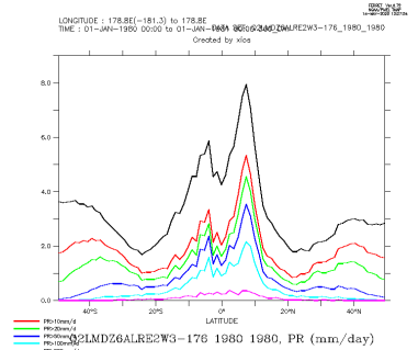
Q2LMDZ6ALRE2W3-176_1980_1980_zon
