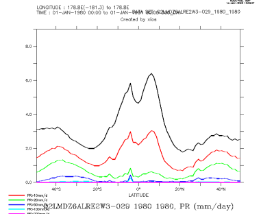
Q2LMDZ6ALRE2W3-029_1980_1980_zon
