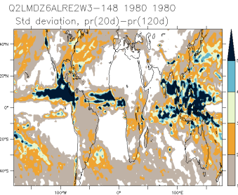
Q2LMDZ6ALRE2W3-148_1980_1980_is
