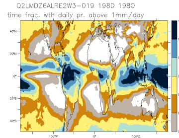
Q2LMDZ6ALRE2W3-019_1980_1980_nd
