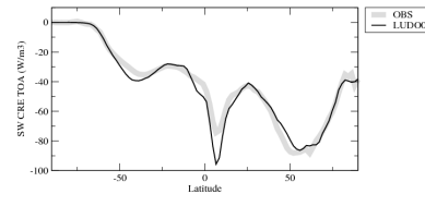
crestzon
