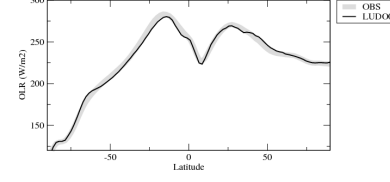
rlutzon
