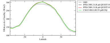
rsdscrezon
