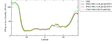
rsuscscrezon
