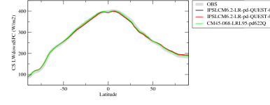
rldscscrezon
