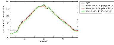
rttson
