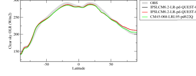
rlutcscrezon
