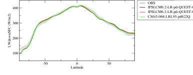
rldscscrezon
