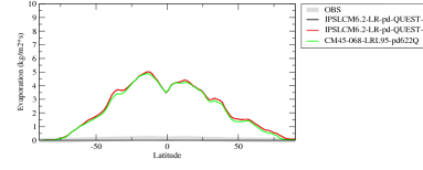
evazon
