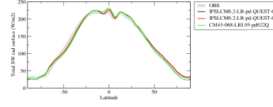
rstscscrezon
