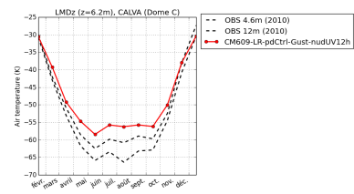
tempDC-CM609-LR-pdCtrl-Gust-nudUV12h
