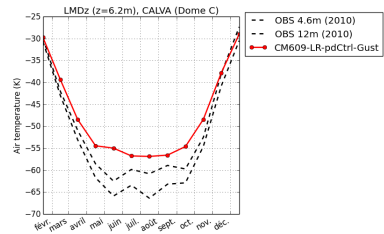
tempDC-CM609-LR-pdCtrl-Gust
