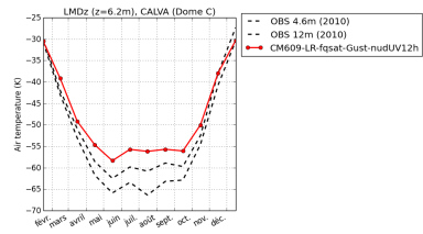
tempDC-CM609-LR-fqsat-Gust-nudUV12h
