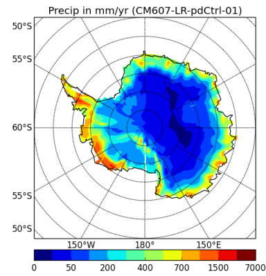
precipSH-CM607-LR-pdCtrl-01
