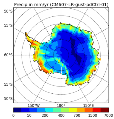
precipSH-CM607-LR-gust-pdCtrl-01
