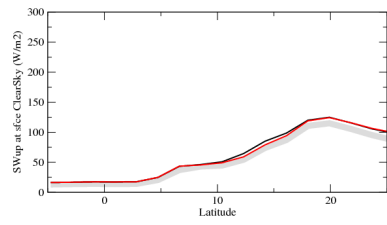
rsuscszn
