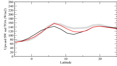
rsutzn
