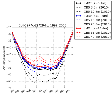
tempDC-CL4-3977c-L2729-frz_1999_2008
