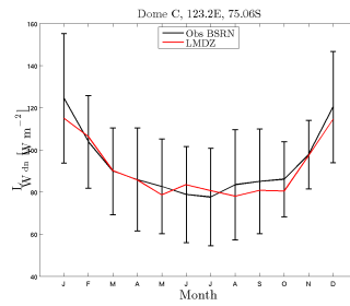
LWdn_DC_CL4.3977c.L2729.frz.frzc1.smtc2_1999_2008
