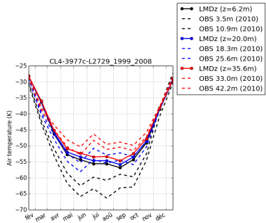
tempDC-CL4-3977c-L2729_1999_2008
