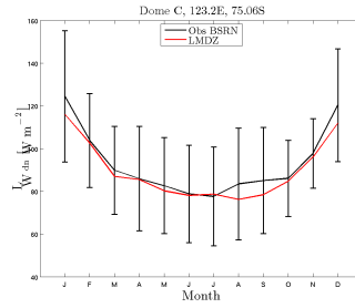
LWdn_DC_CL4.3977c.L2729.frz_1999_2008
