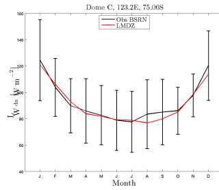
LWdn_DC_CL4.3977c.L2729_1999_2008
