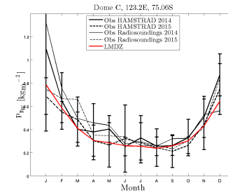
prw_DC_CL4.3977c.L2729_1999_2008
