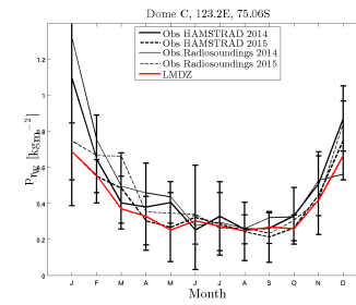
prw_DC_CL4.3977c.L2729.frz.frzc1.smtc2_1999_2008
