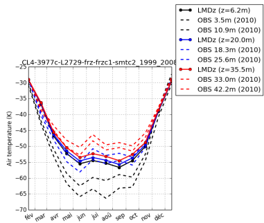
tempDC-CL4-3977c-L2729-frz-frzc1-smtc2_1999_2008
