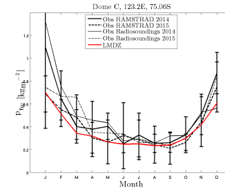
prw_DC_CL4.3977c.L2729.frz_1999_2008
