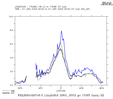
FHLR6014NPv6.0.12splitHd_2001_2003_con
