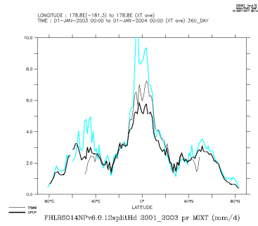
FHLR6014NPv6.0.12splitHd_2001_2003_mix
