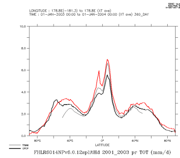
FHLR6014NPv6.0.12splitHd_2001_2003_tot
