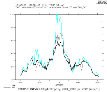
FHLR6014NPv6.0.12splitHalpbug_2001_2003_mix
