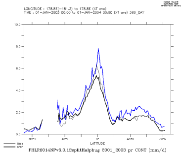
FHLR6014NPv6.0.12splitHalpbug_2001_2003_con
