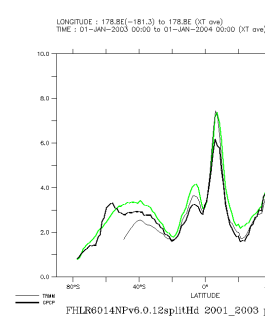
FHLR6014NPv6.0.12splitHd_2001_2003_con
