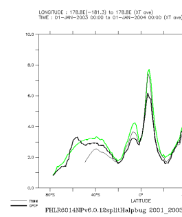
FHLR6014NPv6.0.12splitHalpbug_2001_2003_con
