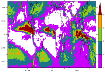
FHLR6014NPv6.0.12splitH 2001 2003 Std deviation, pr(1d)-pr(30d)
