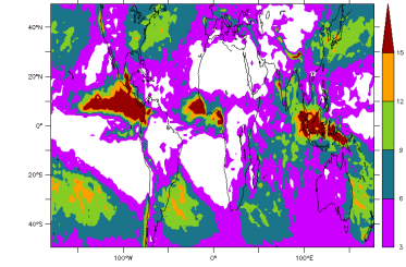
FHLR6014NPv6.0.12splitHalpbug 2001 2003 Std deviation, pr(1d)-pr(30d)
