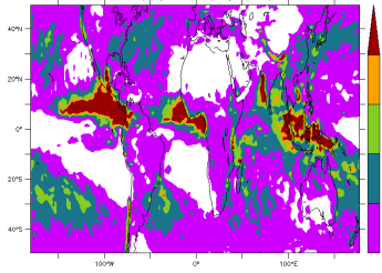
FHLR6014NPv6.0.12splitHd 2001 2003 Std deviation, pr(20d)-pr(120d)
