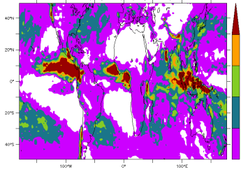
FHLR6014NPv6.0.12splitH 2001 2003 Std deviation, pr(20d)-pr(120d)
