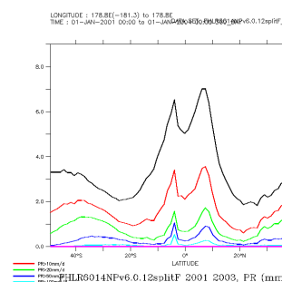
FHLR6014NPv6.0.12splitF_2001_2003_zon
