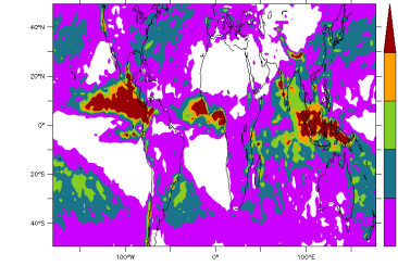
FHLR6014NPv6.0.12splitHalpbug 2001 2003 Std deviation, pr(20d)-pr(120d)
