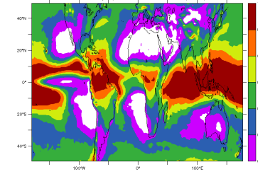
FHLR6014NPv6.0.12splitH 2001 2003 time frac. with daily pr. above 1mm/day
