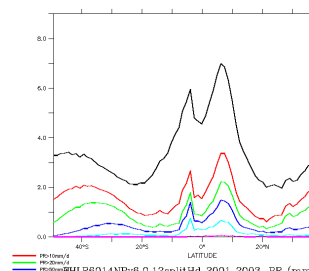
FHLR6014NPv6.0.12splitHd
