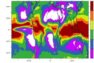
FHLR6014NPv6.0.12splitHd 2001 2003 time frac. with daily pr. above 1mm/day
