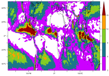
FHLR6014NPv6.0.12splitHd 2001 2003 Std deviation, pr(1d)-pr(30d)
