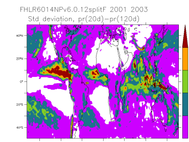
FHLR6014NPv6.0.12split_2001_2003_is
