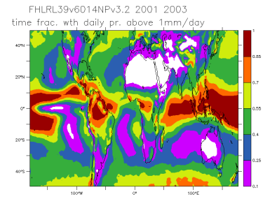
FHLRL39v6014NPv3.2_2001_2003_nd
