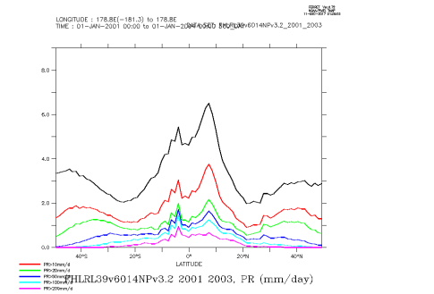
FHLRL39v6014NPv3.2_2001_2003_zon
