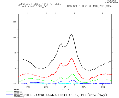
FHLRL39v6014AR4_2001_2003_zon
