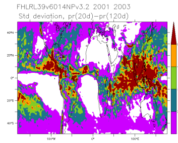
FHLRL39v6014NPv3.2_2001_2003_is
