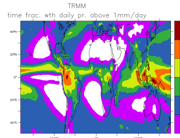
TRMM_nd
