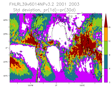
FHLRL39v6014NPv3.2_2001_2003_hf
